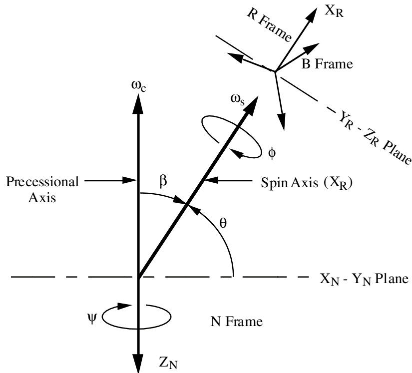
Figure 1 - SPIN-CONE Geometry
